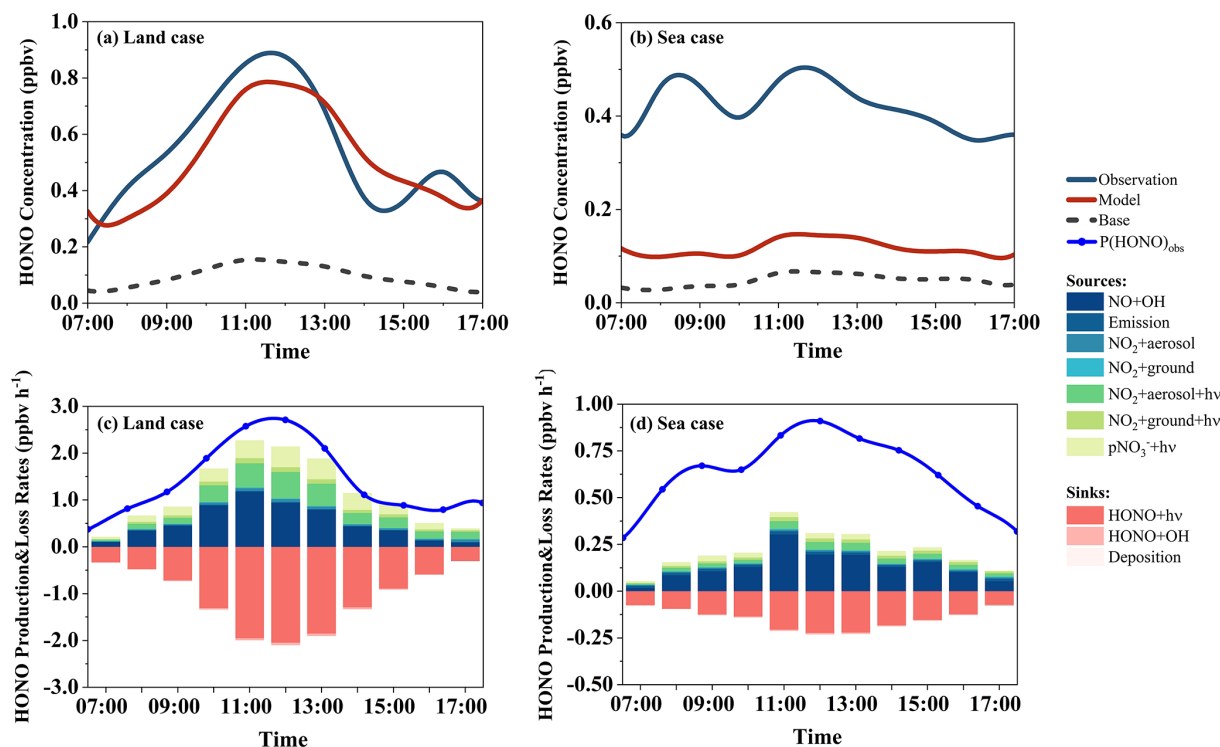
Figure 6. Comparison of the observed and modeled daytime (07:00–17:00) HONO concentrations and modeled HONO budgets in the land case (a, c) and the sea case (b, d).
