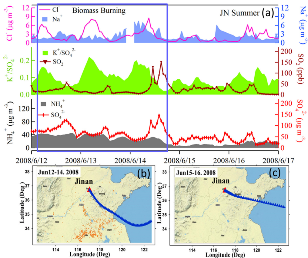
Fig. 6. (a) Time series of air pollutants observed in summer in Jinan and corresponding fire counts over east-central China from Aqua and Terra MODIS: (b) 12 to 14 June 2008; (c) 15 to 16 June 2008.
