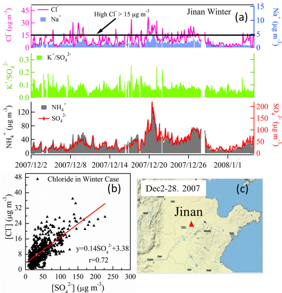
Fig. 5. (a) Time series of air pollutants observed in winter in Jinan, (b) Scatter plot of Cl^- and SO_4^{2-} in winter and (c) corresponding fire counts over east-central China from Aqua and Terra MODIS.
