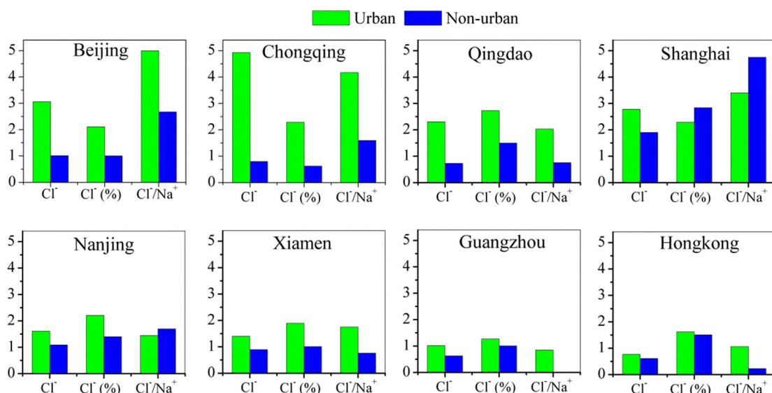
Fig. 4. Comparison of chloride concentration ( \mu\text{g m}^{-3} ), percentage of chloride in \text{PM}_{2.5} , \text{Cl}^- % and \text{Cl}^-/\text{Na}^+ mass ratio at paired urban/non-urban sites in representative cities.
