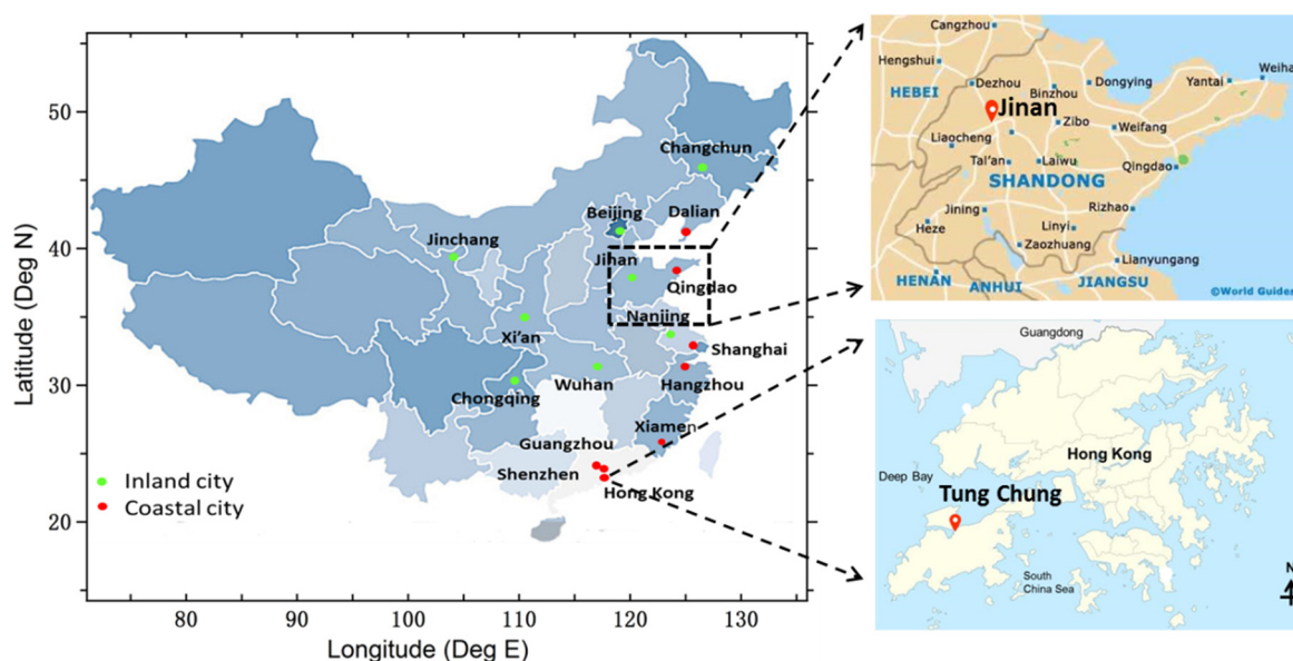
Fig. 1. Left: Locations of the 16 large cities for which particulate chloride concentrations were measured and compiled in this study. Eight coastal cities (at least 100 km from the nearest coastline) are marked in red, and eight inland cities (at least 100 km from the nearest coastline) are marked in green. Right: locations of the sampling sites in Jinan and Hong Kong (Tung Chung). (For interpretation of the references to colour in this figure legend, the reader is referred to the web version of this article.)
