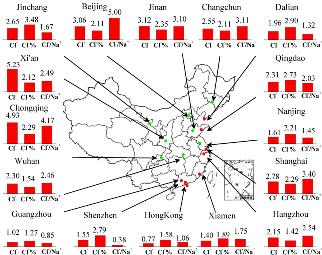
Fig. 3. Spatial distributions of chloride at urban locations in China. Average chloride concentration (µg m -3 ), percentage of chloride in PM 2.5 (Cl - %) and Cl - /Na + mass ratio are indicated. Inland and coastal cities are marked in green and red, respectively. (For interpretation of the references to colour in this figure legend, the reader is referred to the web version of this article.)
